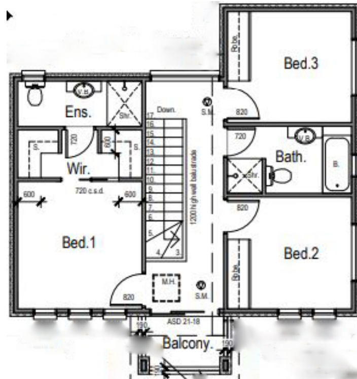
Level 1 Plan
